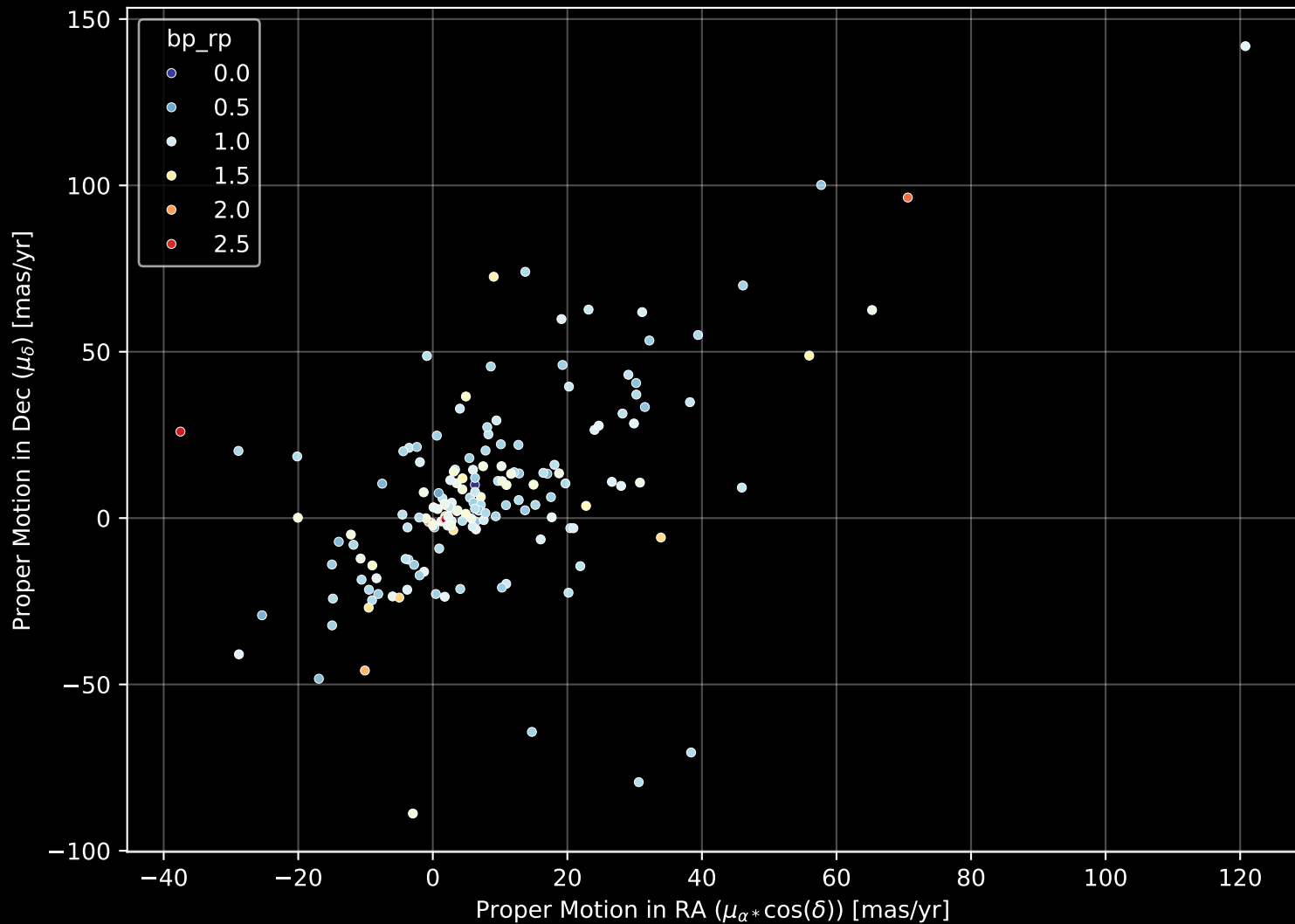
APOGEE DR17 Field: [278-39-O_TESS] Proper Motion Diagram (n= 170)
