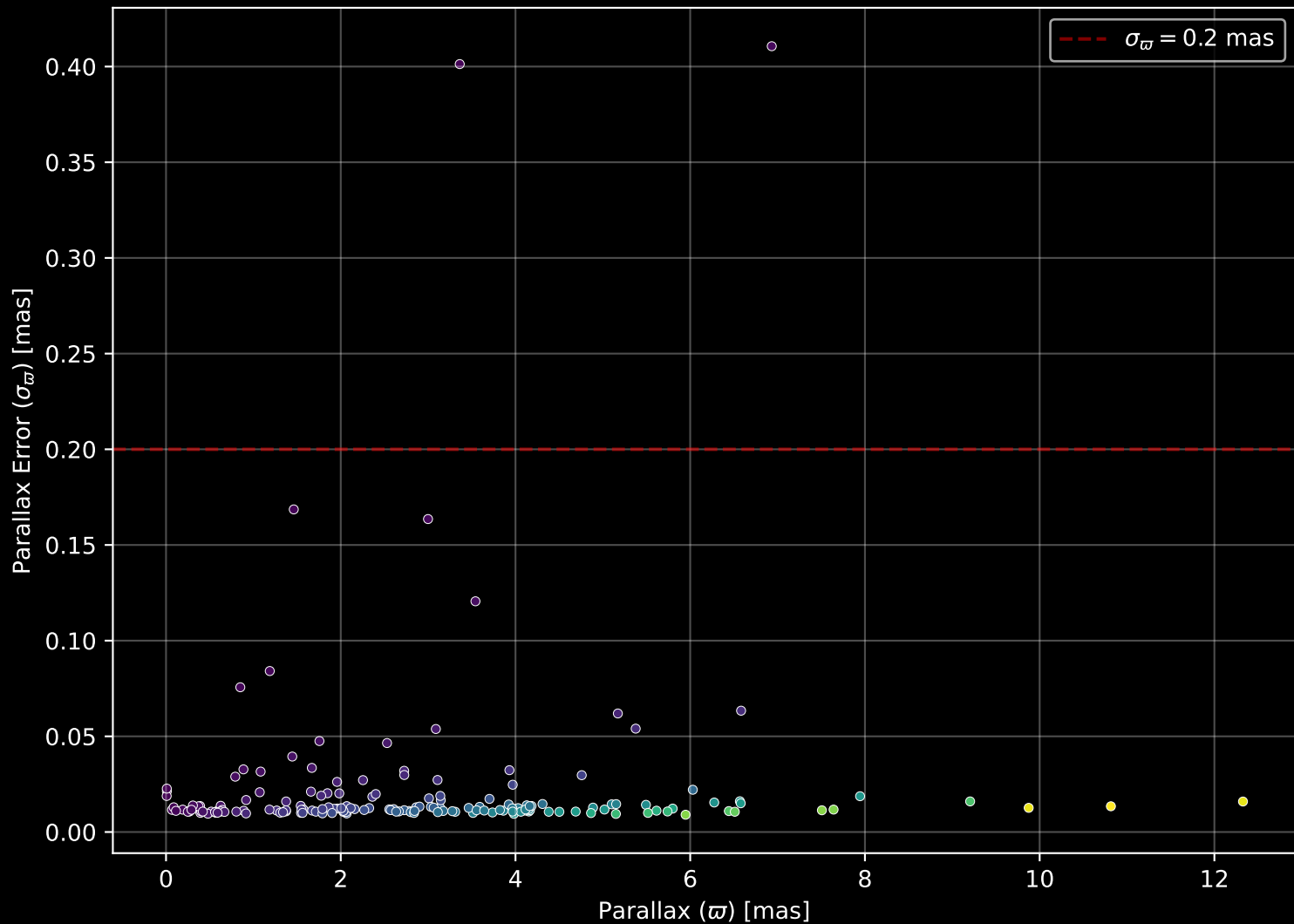
APOGEE DR17 Field: [278-39-O_TESS] Parallax Quality (n= 170)
