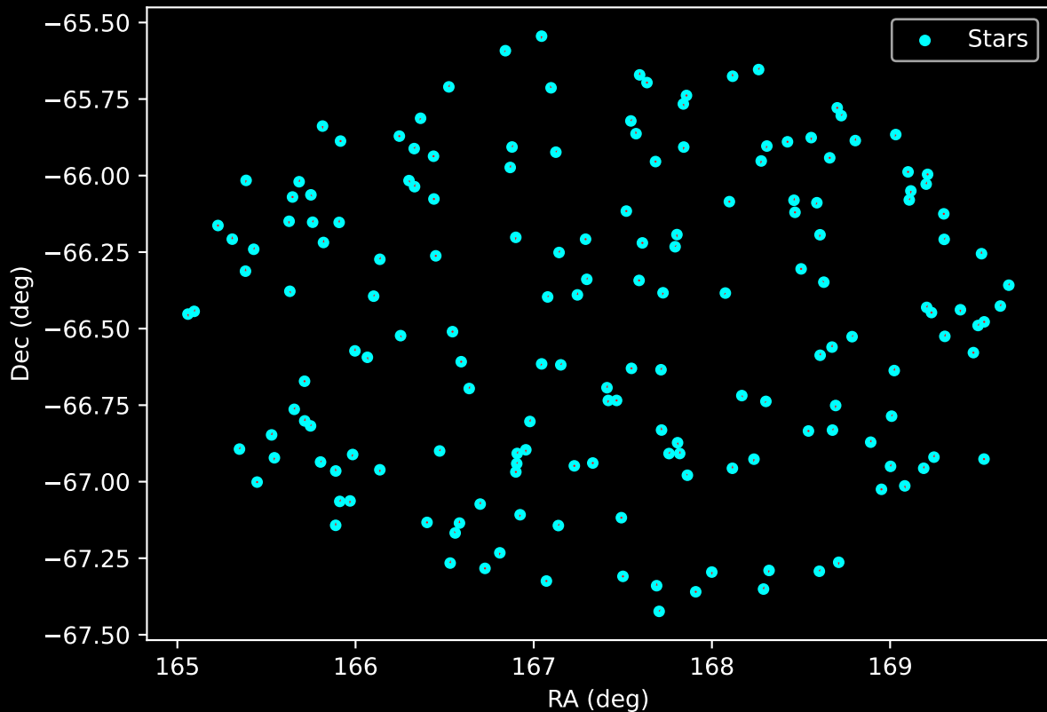
APOGEE DR17 Field: [278-39-O_TESS] Proper Motion Vectors for Gaia Star Field (n= 170)
