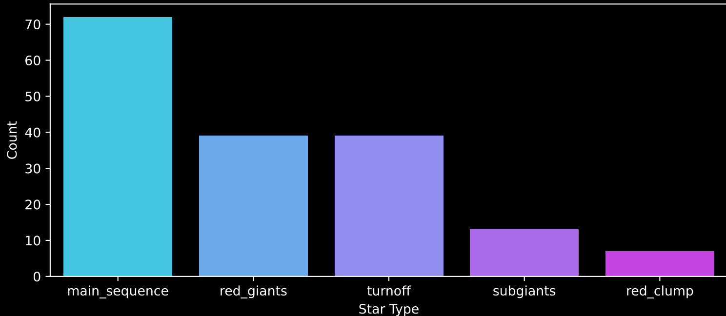
APOGEE DR17 Field: [278-39-O_TESS] Count plot of Star Type
