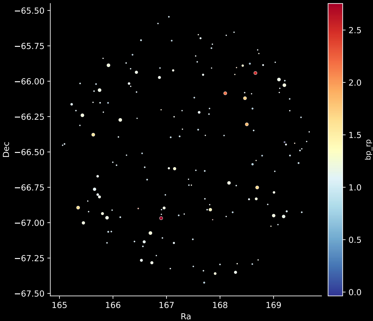
APOGEE DR17 Field: [278-39-O_TESS] Stars: 170
