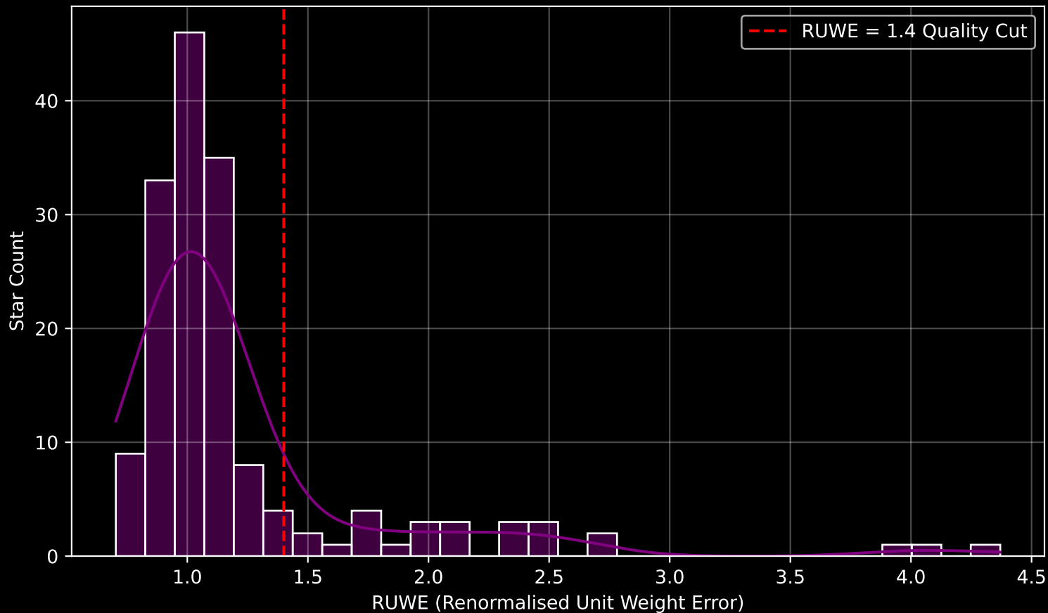
GAPOGEE DR17 Field [278-39-O_TESS] RUWE Distribution (n= 160)
