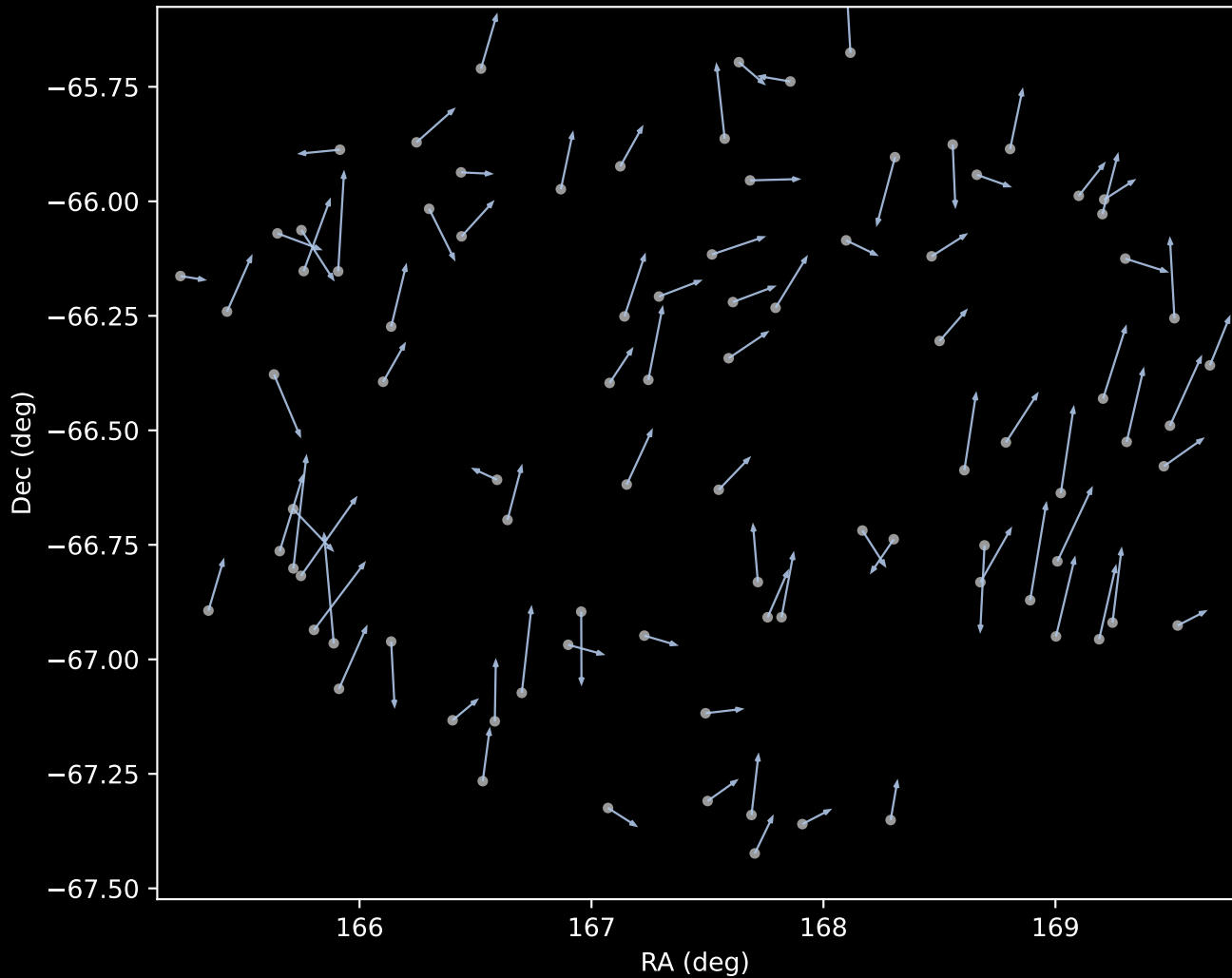
APOGEE DR17 Cluster 1 Proper Motion Vectors (n=90)
