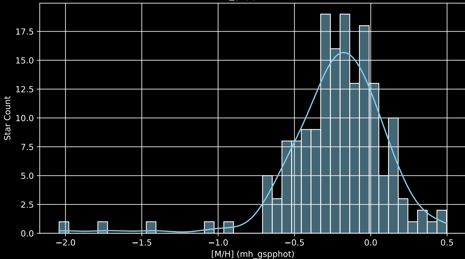
APOGEE DR17 Field: [278-39-O_TESS [M/H] (mh_gspphot) (n= 169)
